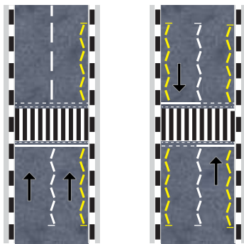
Pedestrian crossing on a dual-carriageway
